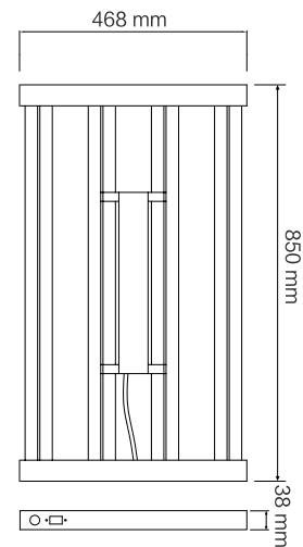
Dimension
