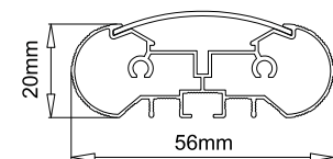
Dimension
